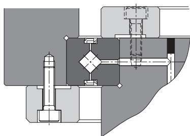
Example of Assembling Model RE
