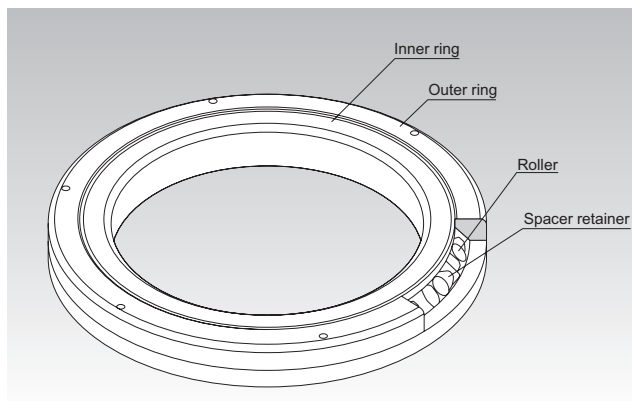
Structure of Cross-Roller Ring Model RB
