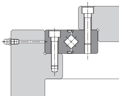
Example 2 of assembling model RU
